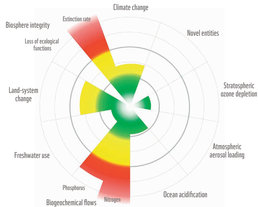
Figure 30: Planetary Boundaries
