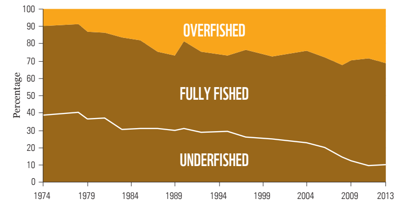
Figure 28: Global trends in the state of world marine fish stocks since 1974
