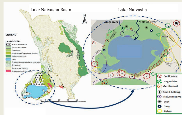
Figure 46: Land use in the Naivasha Basin (WWF, 2011)
